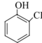
o-chlorophenol
