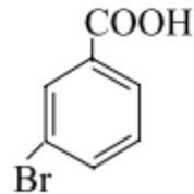
m-bromobenzoic acid
