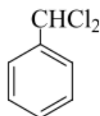
Benzalchloride
