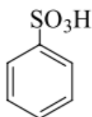
Benzenesulfonic acid
