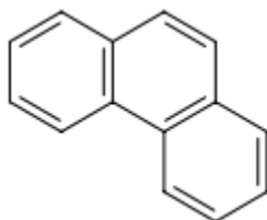
Phenanthrene n = 3 4(3) + 2 = 14 \pi \text{es}
