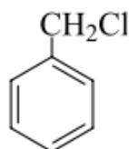
Benzylchloride
