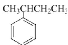
2-Phenylbutane
