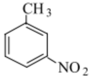
m-nitrotoluene
