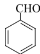
Benzaldehyde
