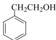
2-Phenylethanol
